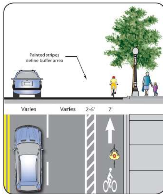
Recommended buffered bike lane design.
