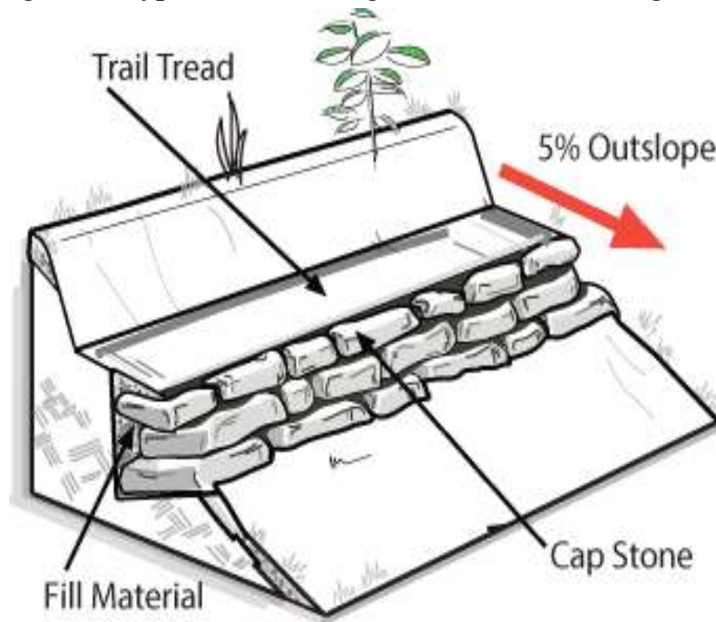
Figure 42: Typical MPOS Design for Natural Retaining Walls
