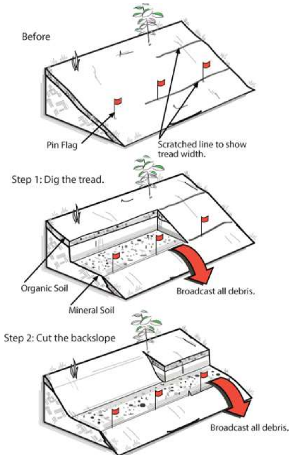
Figure 39: Typical MPOS Singletrack Full Bench Trail
