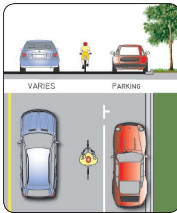
Example of on-street parking delineation.
