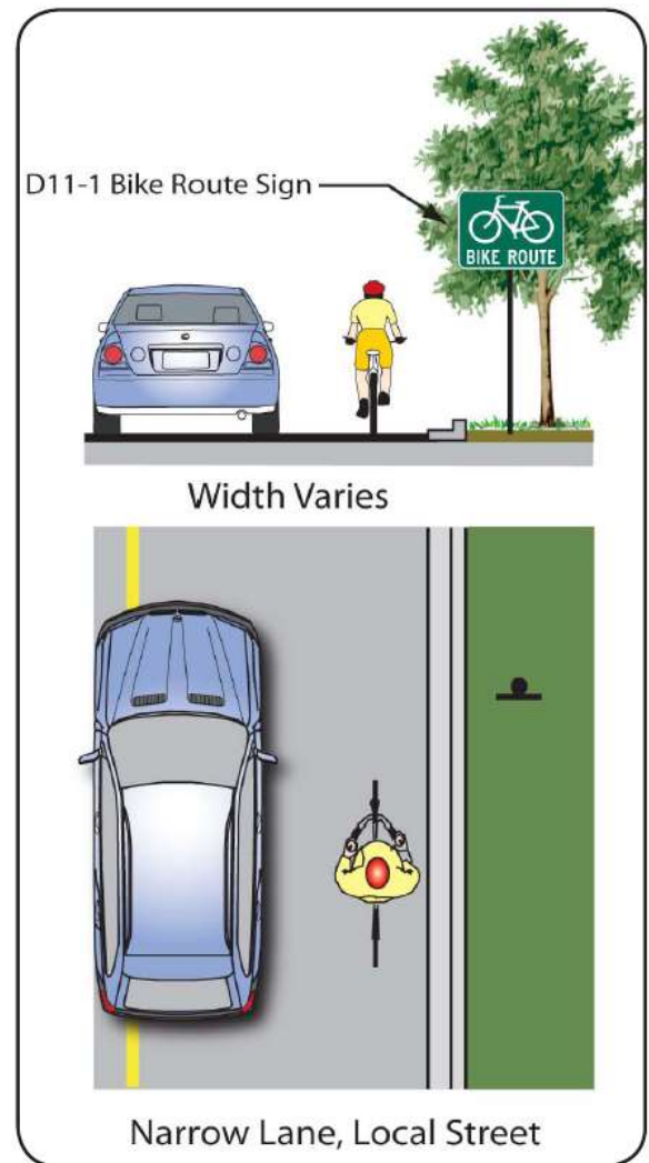
Recommended design for bike routes/ bicycle boulevards.
