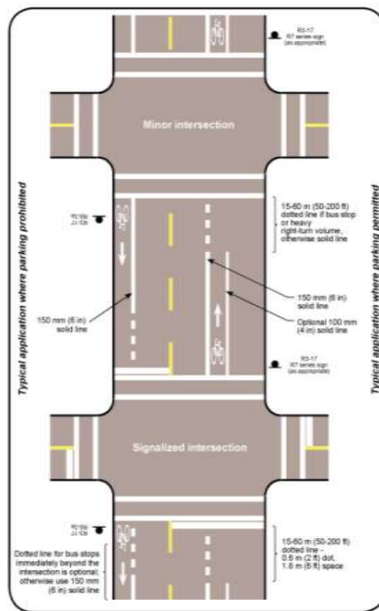
Typical pavement markings for bike lane on two-way street (AASHTO)
