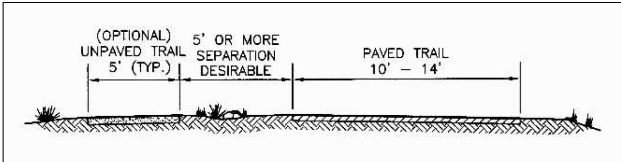
Figure 37: Typical Paved Multi-Use Trail Cross Section
