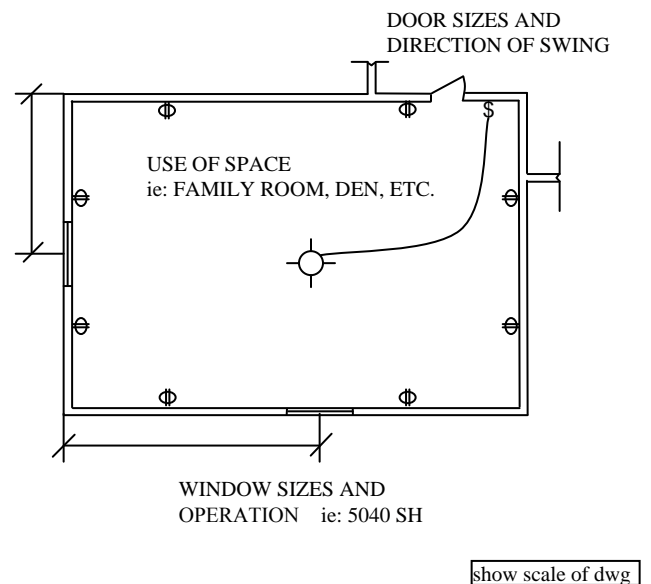
Figure No. 3 FLOOR PLAN
