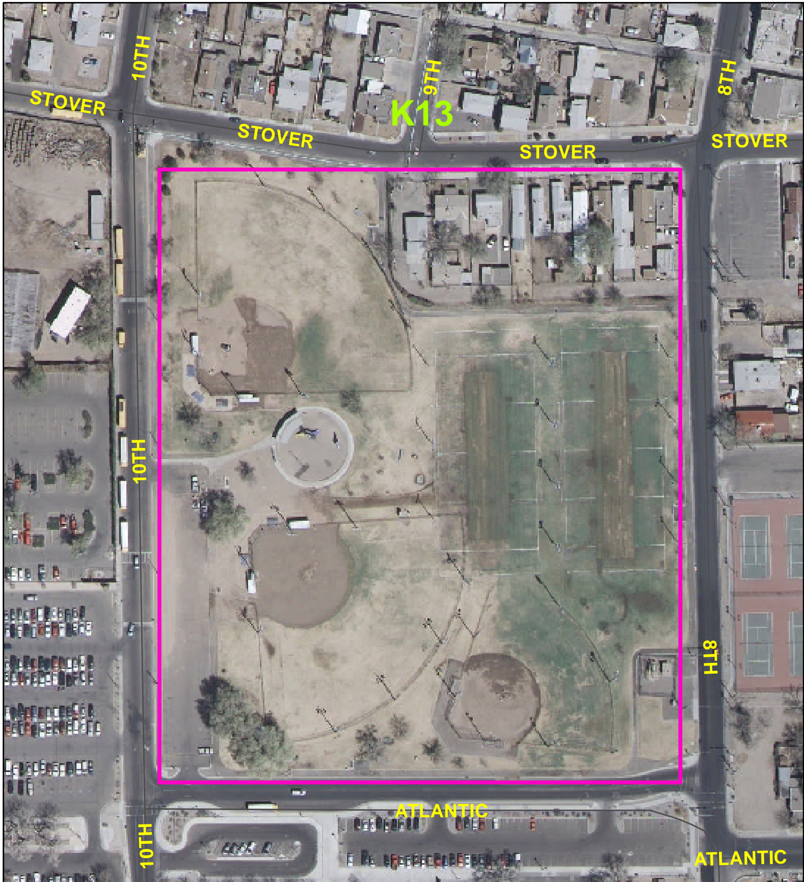
TINGLEY PARK : A 14 ACRE FLOOD CONTROL / PARK FACILITY DESIGNED BY WILLISON&CO COSTRUCTED BY NM UNDERGROUND MARCH TO JULY 2007
