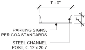
6 PARKING SIGN - SECTION 1" = 1'-0"
