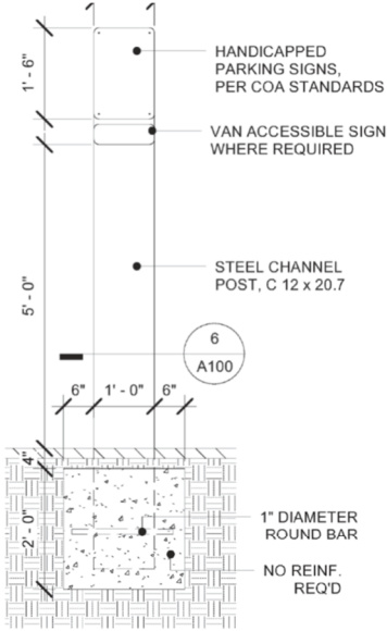
7 PARKING SIGN 1/2" = 1'-0"
