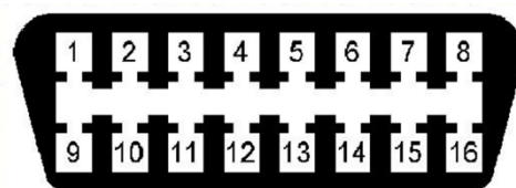
OBD-II pin numbering
