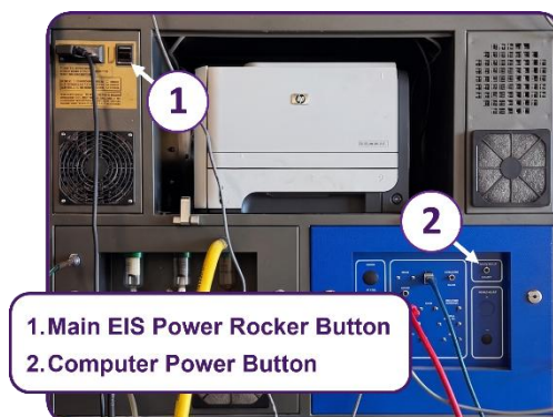
Analyzer start-up controls
