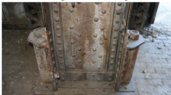
Bay #4 columns supported on deep piles, dampened by springs.
