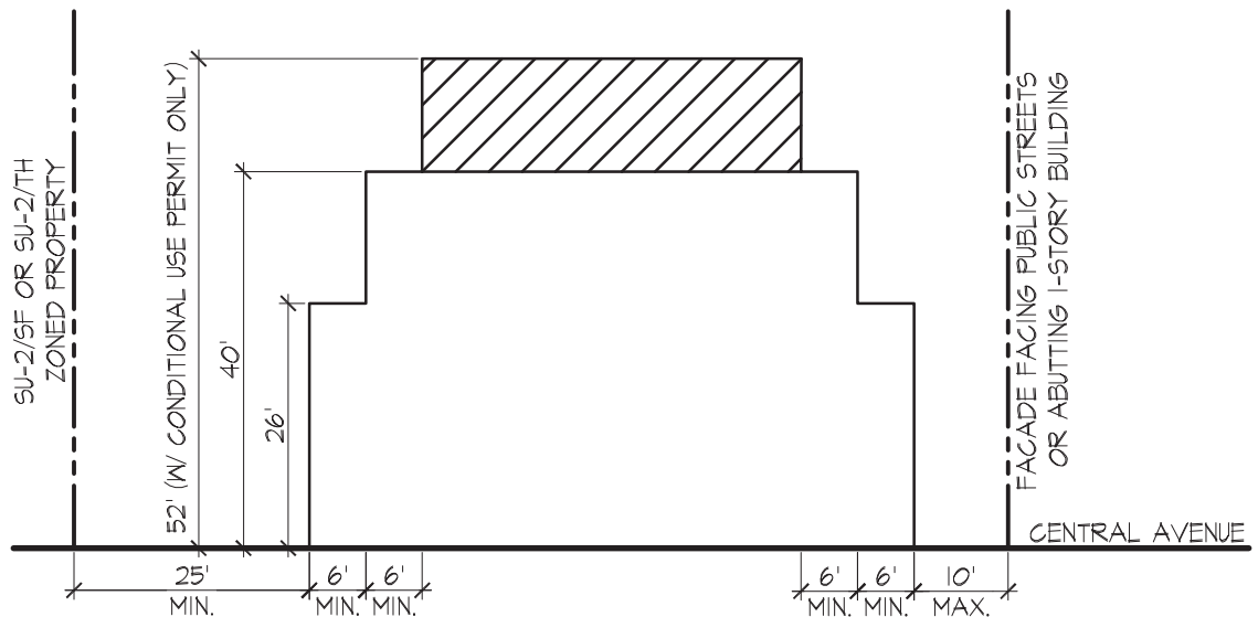
Building Height and Stepbacks for Facades
