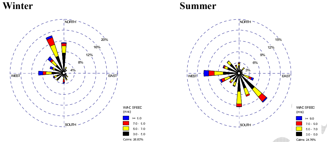
Figure 2: Seasonal Wind Roses for Albuquerque
