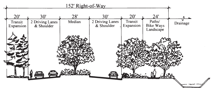
Cross Section
