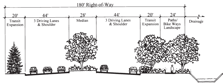
Cross Section
