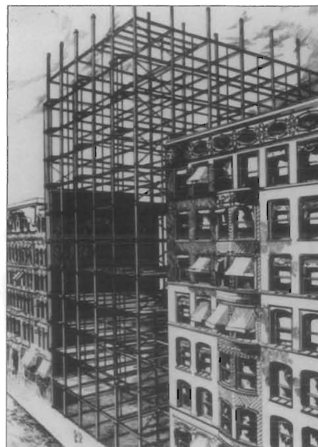
Iron and Steel Skeleton Frame, Unity Building, Chicago, Illinois, 1891-1892 (Clinton J. Warren, architect). The development of the skeleton frame was pioneered by architects of the "Chicago School" in the late-19th century. With this method the weight of the building is carried on the frame, not the walls, allowing the construction of taller buildings without increasing the wall thickness.
