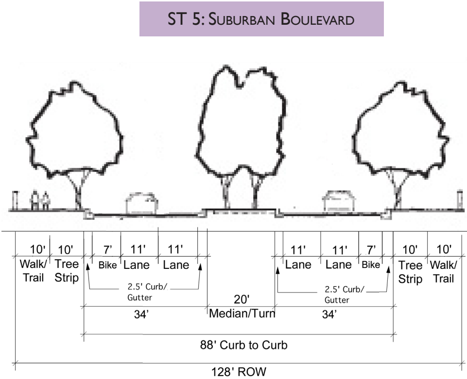
EXHIBIT 10.11 – STREET TYPE 5: SUBURBAN BOULEVARD
