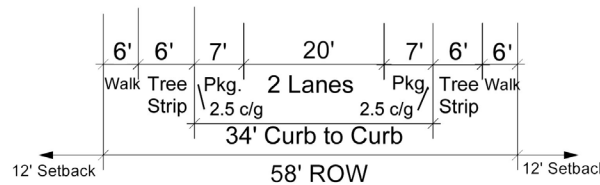
STREET TYPE 1.2 – TYPICAL RESIDENTIAL COLLECTOR (2 LANES)
