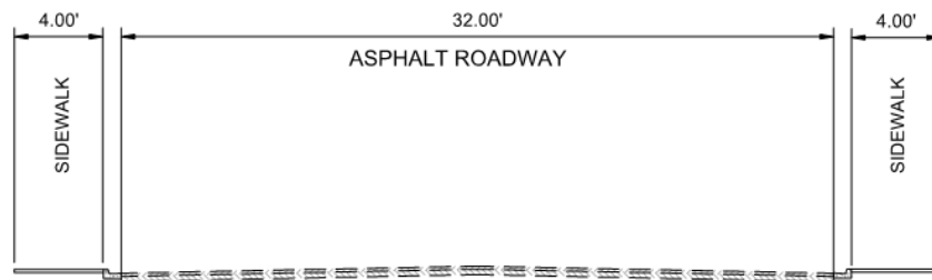
Figure 5: Santa Clara Avenue Existing Typical Section
