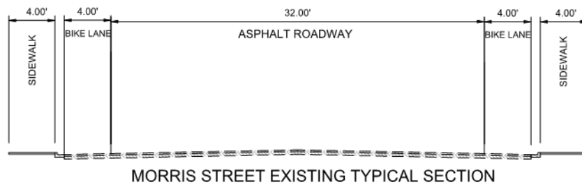
Figure 5: Morris Street Existing Typical Section
