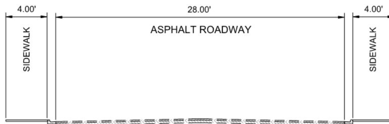
Figure 5: Eastern Avenue Existing Typical Section
